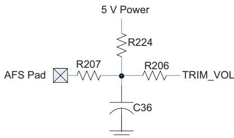
Figure 2-12. TRIM_VOL
