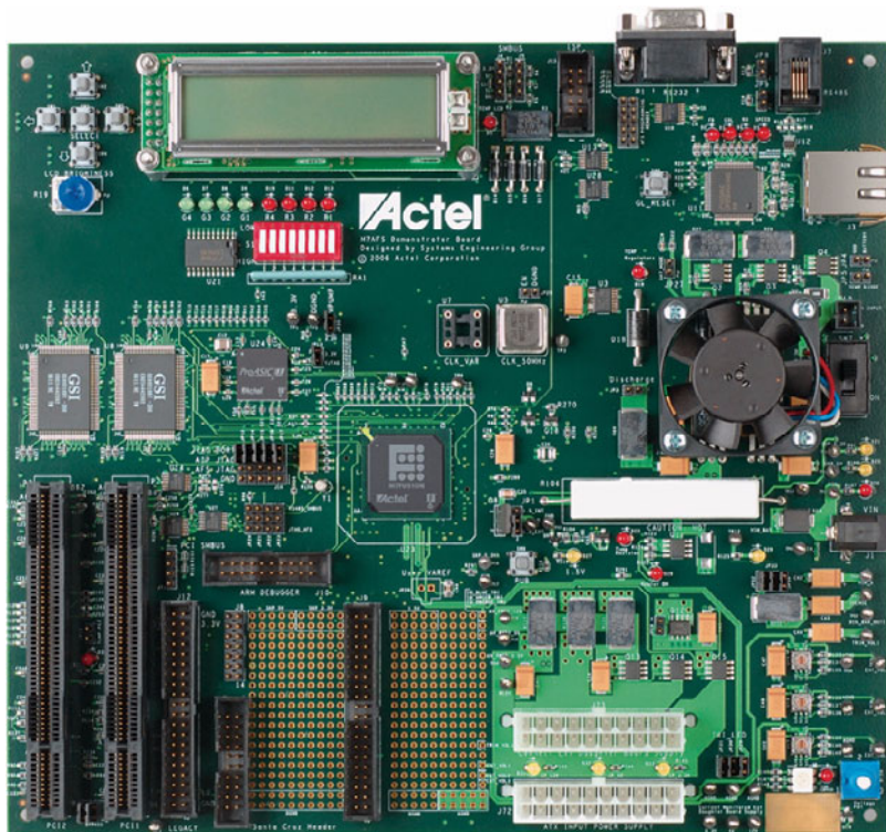
Figure 1. System Management Board
