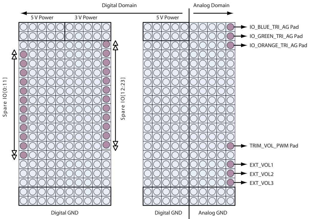
Figure 2-14. Prototype Section
