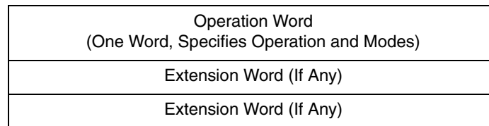
Figure 2-1. Instruction Word General Format
